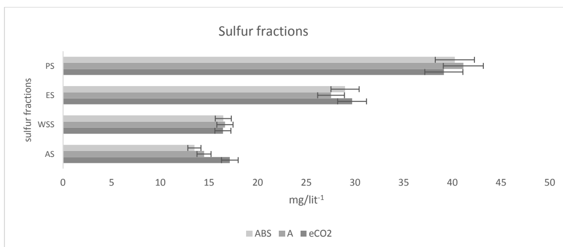
Fig. 2. Distribution of sulphur fractions Available Sulphur (AS), Water-Soluble Sulphur (WSS), Exchangeable Sulphur (ES), and Precipitated Sulphur (PS) from three different soils elevated, ambient, and ambient bulk soil
