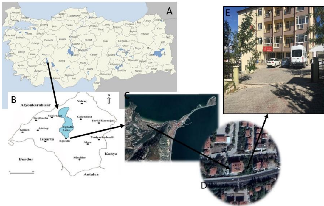
Fig. 1. The aerial view and location of Egirdir Nursing Home (A: The map of Turkiye, B: The map of Isparta province, C: Aerial view of Egirdir town, D: Aerial view of Egirdir Nursing Home, E: Egirdir Nursing Home building)
