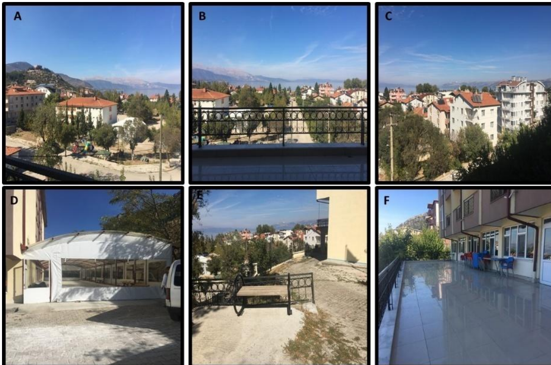
Fig. 3. The location of Egirdir Nursing Home and its open space (A, B, C: Surroundings of nursing home, D: Reserved area for gaming, E: Seating element, F: High terrace)
