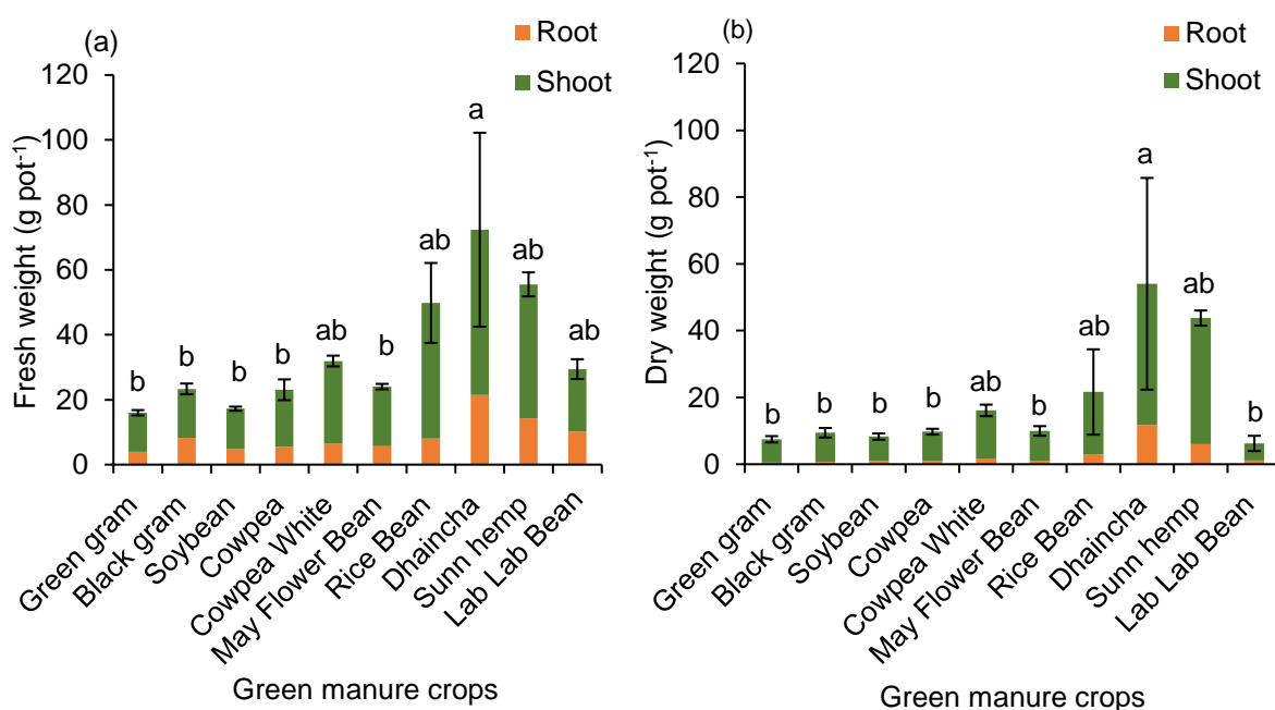
Fig. 1. (a) Fresh weight (g pot -1 ) and (b) Dry weight (g pot -1 ) of GMs at the flowering stage
