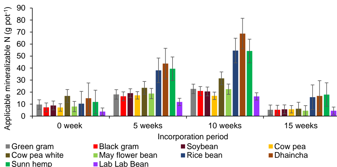
Fig. 3. Applicable mineralizable N (g pot -1 ) from GMs incorporated into the soil
