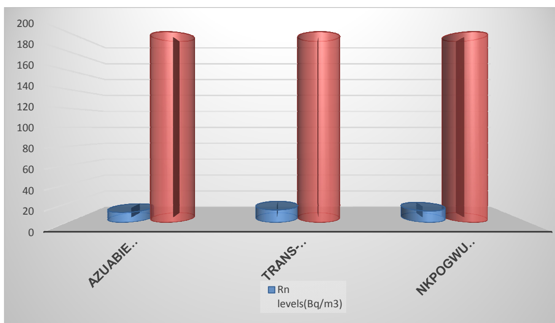
Fig. 2. Average Indoor Radon Level of sample locations and ICPR reference level
