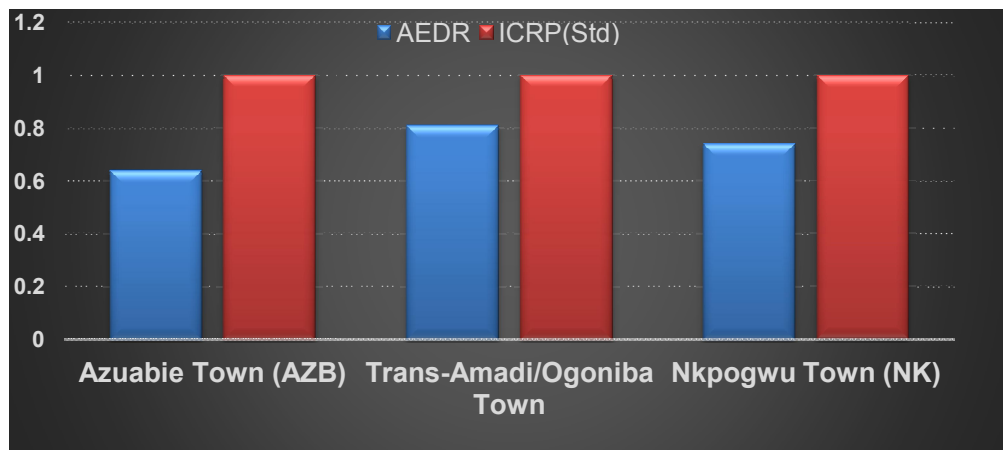
Fig. 4. Annual effective dose rate (AEDR) and ICRP standard
