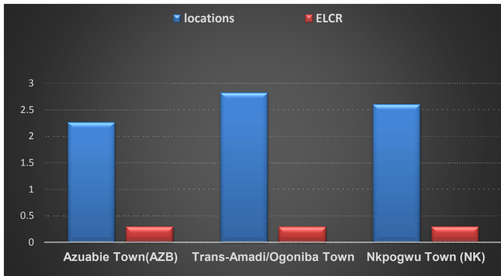
Fig. 5. Excess life time cancer risk (ELCR) of sample locations with world standard
