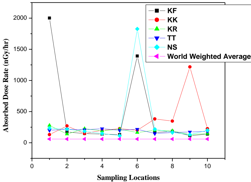
Fig. 3. Comparison of absorbed dose rates and the world weighted average
