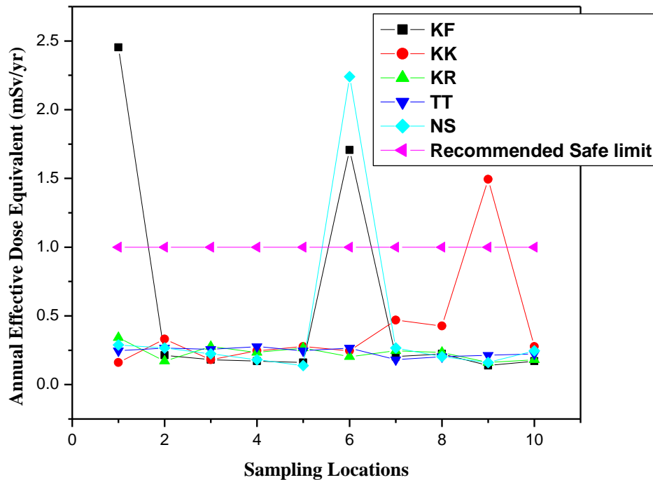
Fig. 4. Comparison of annual effective dose equivalent and the recommended safe limit
