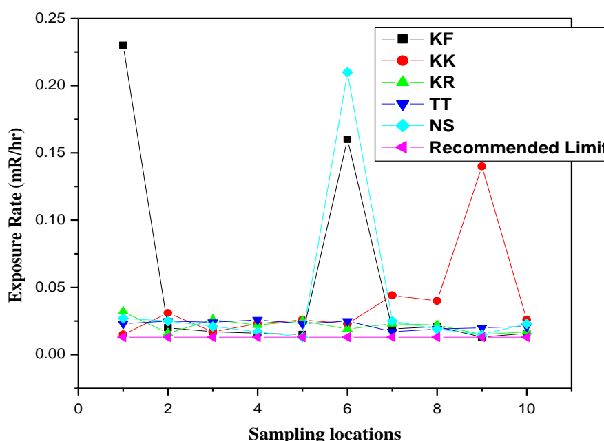
Fig. 2. Comparison of measured outdoor background exposure rates and the recommended limit
