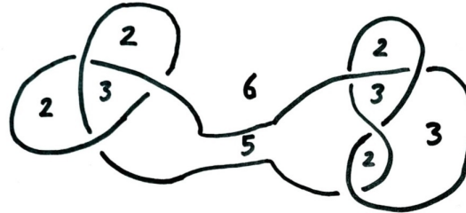
Fig. 5. Connected sum of Fig. 3a and Fig. 3b
