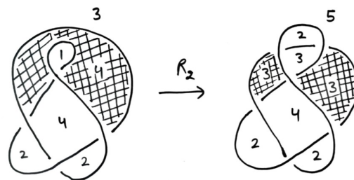
Fig. 12. Example of reverse case of R_2 move
