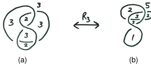
Fig. 14. Example of R_3 move
