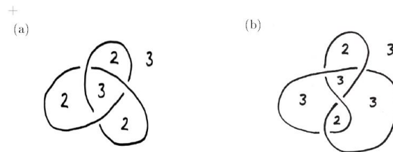
Fig. 3. The region numbering of all the regions of the knot diagrams in Fig. 3
