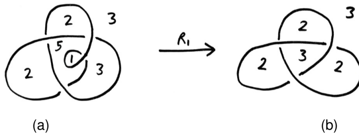
Fig. 8. Example of reverse case of R_1 move
