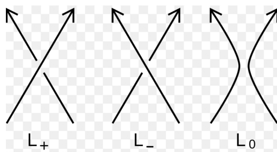
Fig. 1. L_+, L_- , and L_0
