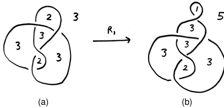
Fig. 7. Example of R_1 move
