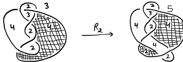
Fig. 11. Example of reverse case of R_2 move
