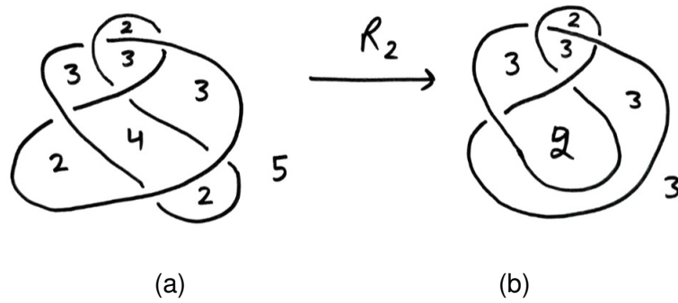
Fig. 10. Example of R_2 move
