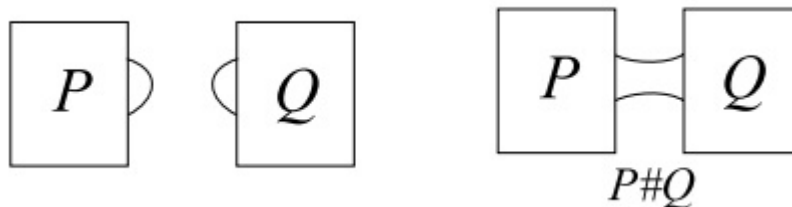
Fig. 4. Connected sum of two knot diagram P and Q
