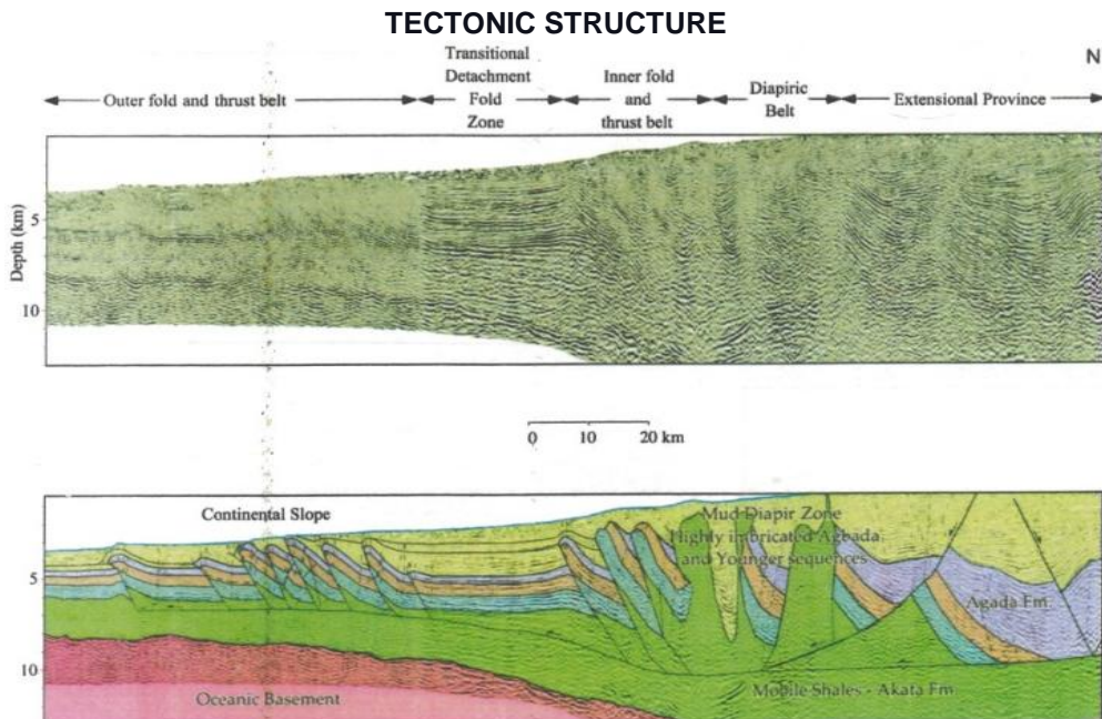
Fig. 4. Tectonic structures drawn over a seismic profile of the Niger Delta Basin
