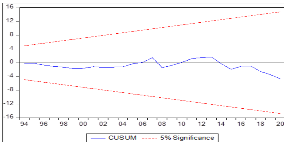
Fig. 2. Plot of cumulative sum of recursive residual
