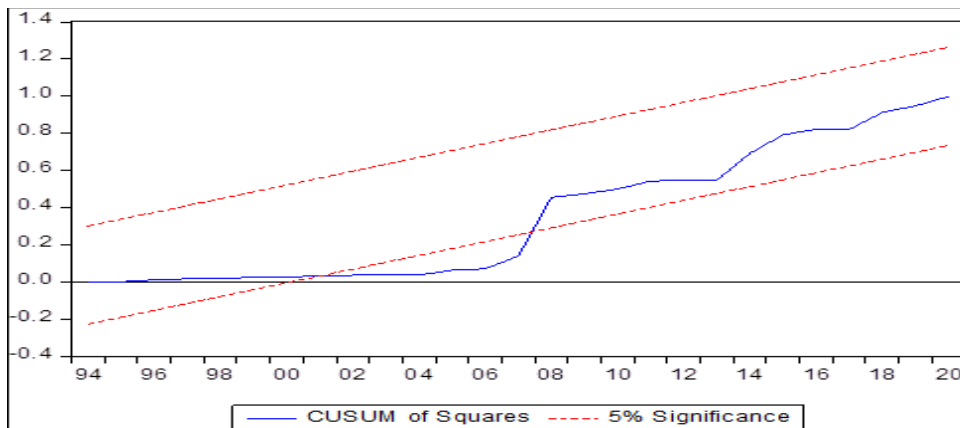
Fig. 3. Plot of cumulative sum squares recursive residual
