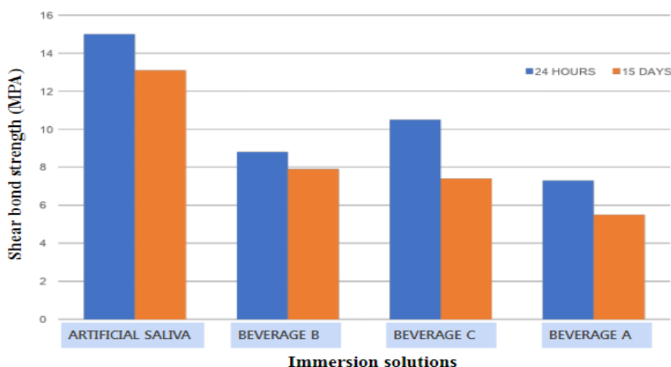
Fig. 3. Effect of types of solution and immersion period on shear bond strength
