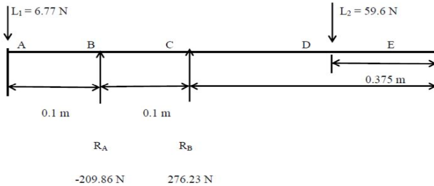
Fig. 4. Force diagram
