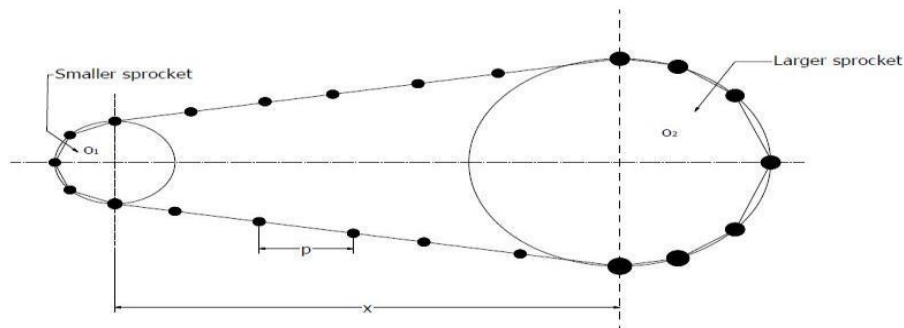
Fig. 2. Schematic drawing of the chain
