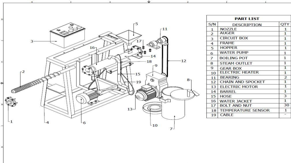
Fig. 1. Exploded view of the modified fish feed extruder
