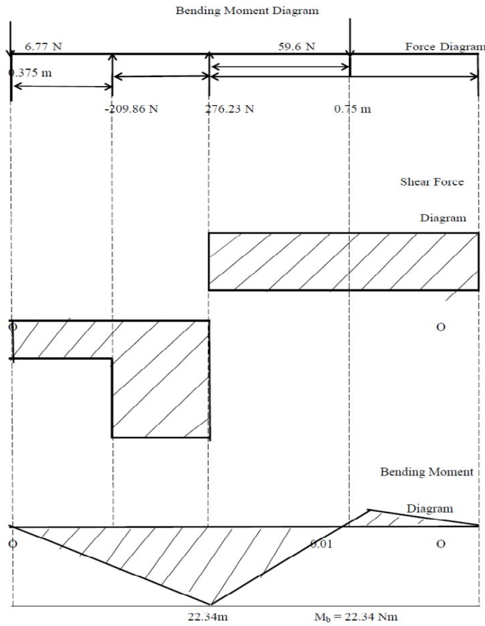
Fig. 4. Bending moment diagram
