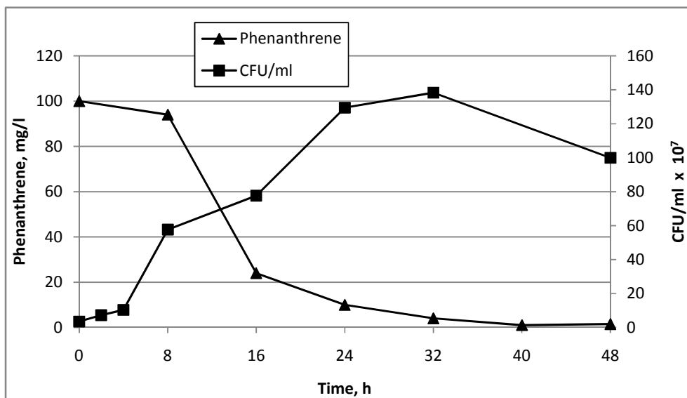
Fig. 1. Phenanthrene degradation and cell proliferation
