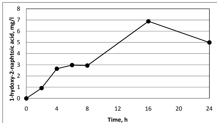
Fig. 4. The accumulation of 1-hydroxy-2-naphthoic acid in course of phenanthrene degradation in the medium with Tween 20 added
