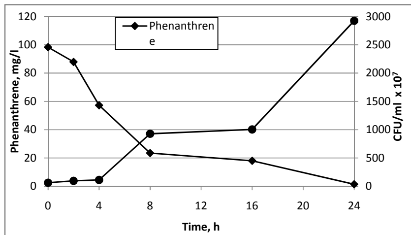
Fig. 3. Phenanthrene degradation and bacterial cell proliferation in the medium with Tween 20 added
