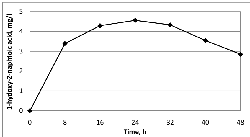
Fig. 2. Accumulation of 1-hydroxy-2-naphthoic acid in course of phenanthrene degradation
