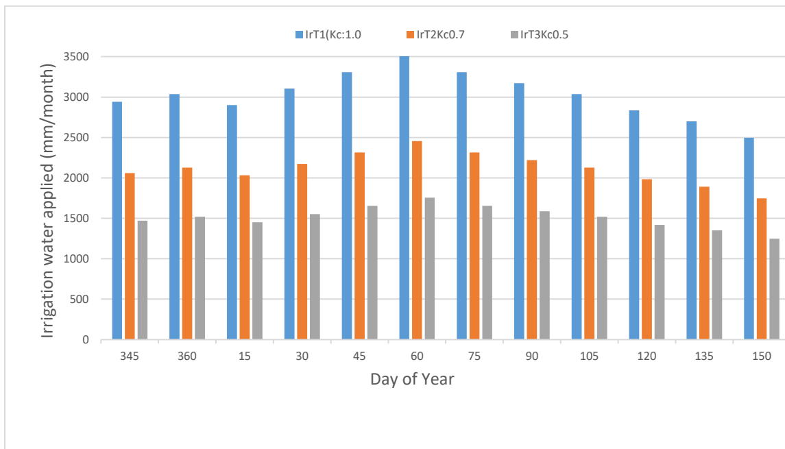
Fig. 2. Time course of irrigation water applied during the period of experiment (December to May). The three irrigation treatments were coded as: IrT1 ( EPan*1.0 kcp), IrT2 (EPan *0.7kcp) and IrT3 (EPan * 0.5 kcp). EPan is Pan evaporation and kcp is Pan
