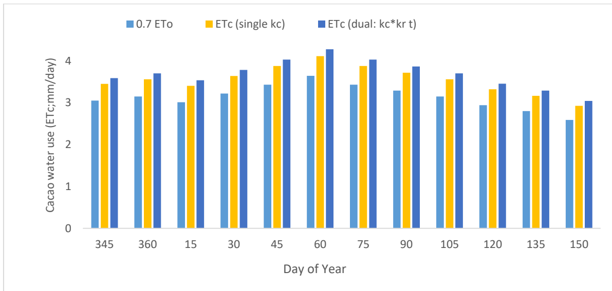
Fig. 5b. Time course of cacao water use (ETc by single and dual kc: kc (1.13), kr t (1.04) IrT1:1.0 EPan and EPan (IrT1; EPan*0.7 Kcp)
