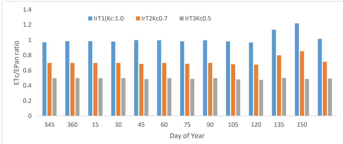
Fig. 6a. Ratio of cacao water use (ETc) to Pan evaporation (EPan) as affected by irrigation regime. The irrigation treatments were coded as: IrT1 (EPan*1.0 kcp), IrT2 (EPan *0.7kcp) and IrT3 (EPan *0.5kcp). EPan is Pan evaporation
