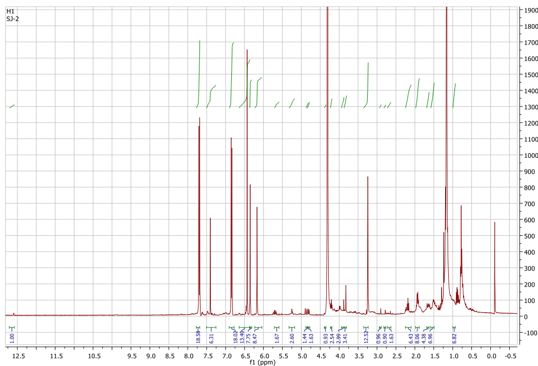
Fig. 4. The 1 H-NMR Spectrum of Apigenin (4', 5, 7-trihydroxyflavone)
