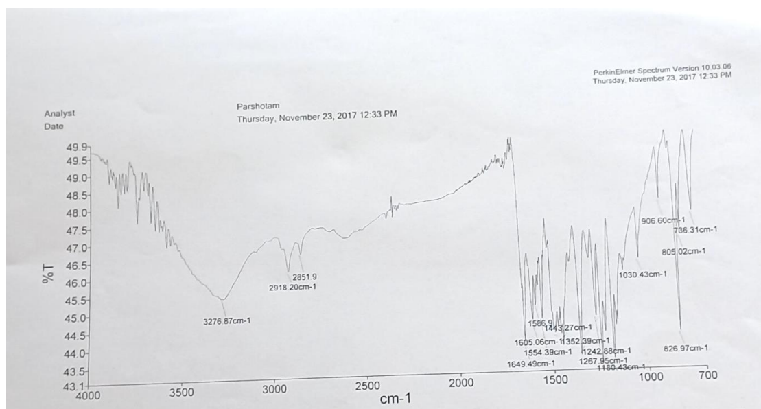
Fig. 3. The IR Spectrum of Apigenin (4', 5, 7-trihydroxyflavone)
