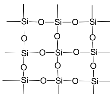
Fig. 1. Structure of Silica
