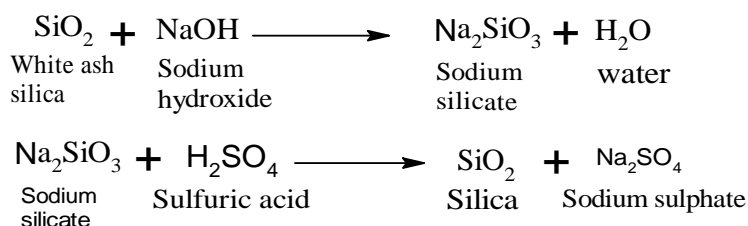
Scheme 1. Reaction for the Production of Silica from Rice Husk Ash
