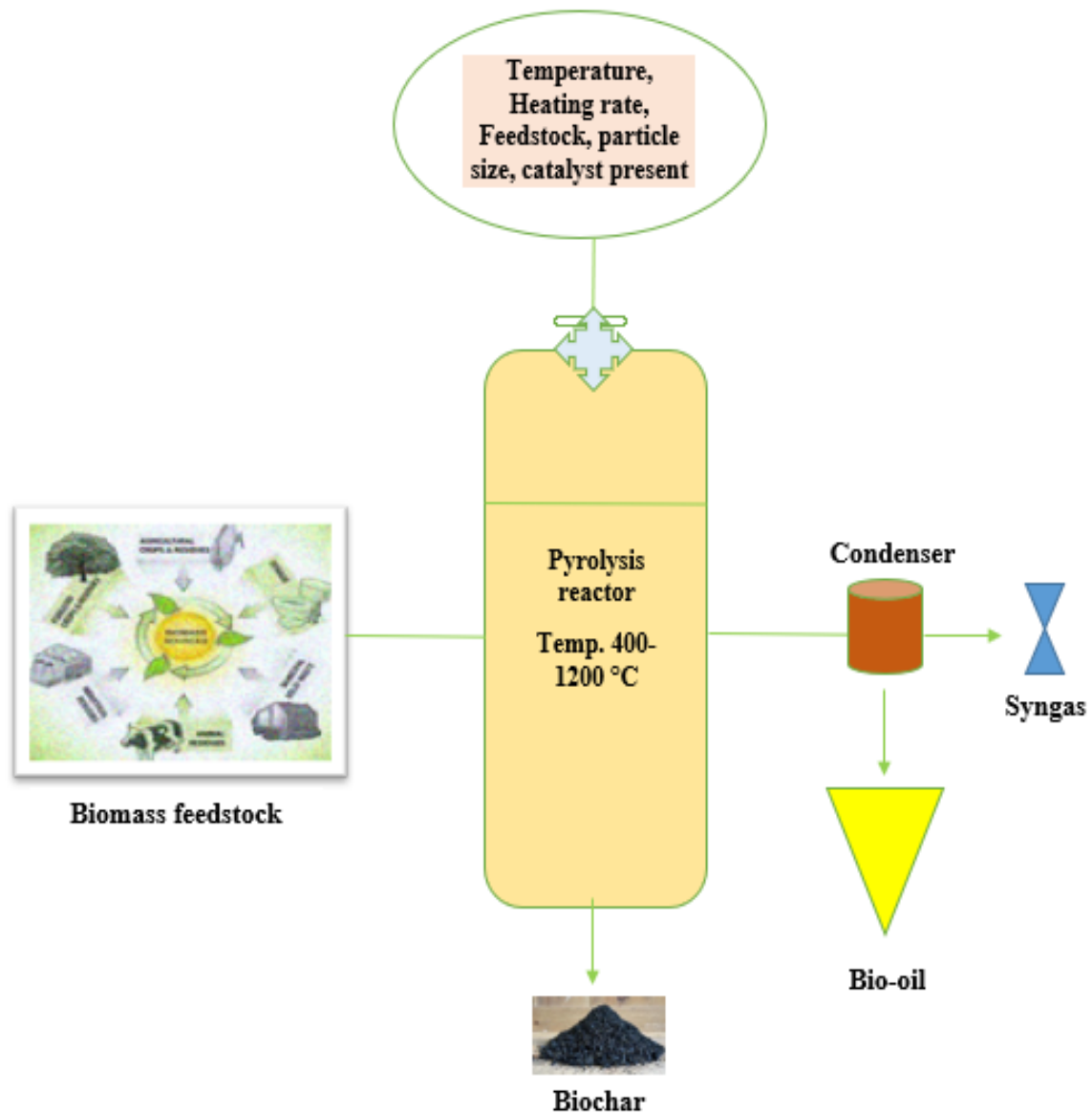
Fig. 1. Production process of biochar by pyrolysis
