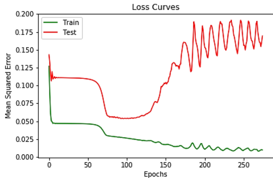
Figure 4. Mean squared error as a function of the number of epochs: a diverging model.
