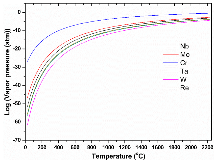
Figure 9. Image indicating the vapor pressure in log as a function of temperature (from room temperature to around 2200 °C).
