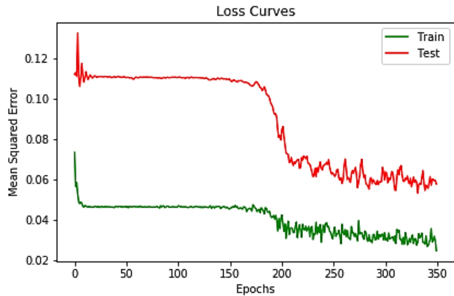
Figure 3. Learning curves of mean squared error as a function of the number of epochs. The red solid red curve represents the average 20-fold cross-validated loss scores on the validation fold, and the green solid curve corresponds to the 20-fold cross-validated loss score on the training data.
