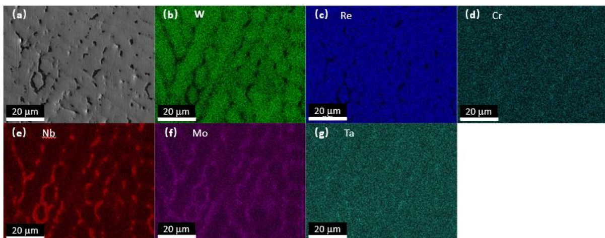
Figure 10. EDS mapping results of the sample C_{0.1}Cr_3Mo_{11.9}Nb_{20}Re_{15}Ta_{30}W_{20} . (a) is the SEM image showing the area for EDS mapping analysis, (b–g) indicate the distribution of W, Re, Cr, Nb, Mo and Ta elements, respectively, on the sample area.
